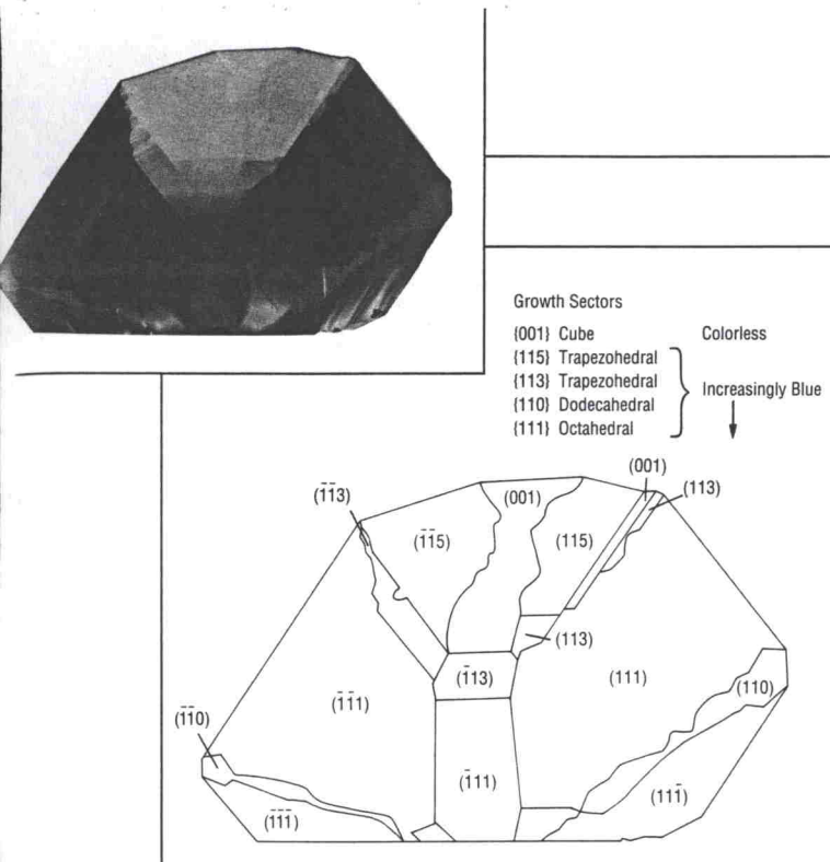
Figure 10. The 0.014-ct synthetic diamond (shown here in the form of a polished plate 0.19 mm thick and 4.2 mm wide) in this transmission optical photomicrograph and growth-sector line drawing was doped with 14 times as much boron as the one shown in figure 9. Infrared spectra (Rooney, 1992) indicate no nitrogen but 0.08 ppm uncompensated boron in the {001} sectors. Similar boron concentrations in other sectors are: {111}—40 ppm, {110}—25 ppm, {113}—9 ppm, and {115}—4 ppm. Photo by C. M. Welbourn.
