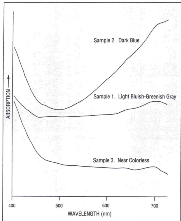
Figure 6. The visible spectra of all three faceted synthetic diamonds, recorded at liquid-nitrogen temperature, show increasing absorption toward the ultraviolet. For samples 1 and 2, weak or moderate increasing absorption is also evident toward the infrared. In contrast to the other two samples, the stronger increasing absorption at the long-wavelength end of its spectrum gives rise to the darker blue color of sample 2.
