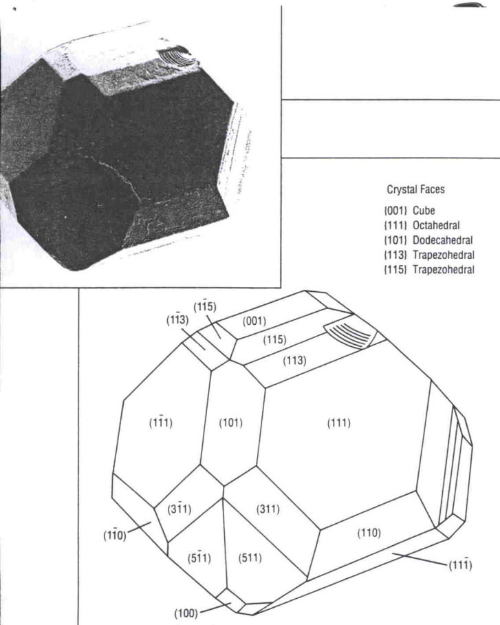
Figure 8. This low-magnification scanning electron micrograph and line drawing of a small boron-doped synthetic diamond crystal show the arrangement of crystal faces. Note the additional \{115\} trapezohedral faces lying between the \{113\} faces and the top \{001\} face.
