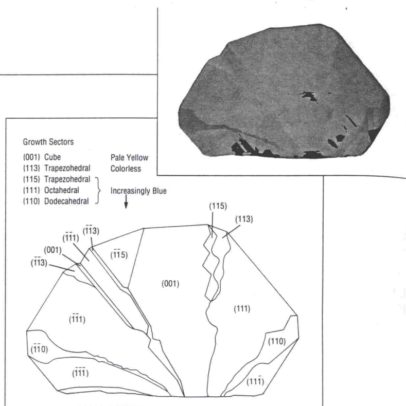
Figure 9. A transmission optical photomicrograph and growth-sector line drawing of a 0.075-ct boron-doped synthetic diamond in the form of a polished plate (0.55 mm thick, 3.9 mm wide). The \{001\} growth sector is pale yellow. The \{113\} sectors are essentially colorless. The remaining sector types are all blue, with the intensity of color increasing in the order \{115\} , \{111\} , \{110\} . Infrared measurements (Rooney, 1992) indicate that the yellow color in the \{001\} sectors resulted from its being type Ib (nitrogen concentration of about 11 ppm). For the blue type IIb regions, the concentration of uncompensated boron was approximately 0.55 ppm for \{115\} , 1.1 ppm for \{111\} , and 2.2 ppm for \{110\} sectors. Photo by C. M. Welbourn.
